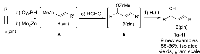
Scheme 2. One-pot synthesis of 2-B(pin)-substituted allylic alcohols through 1-alkenyl-1,1-heterobimetallic intermediates.
